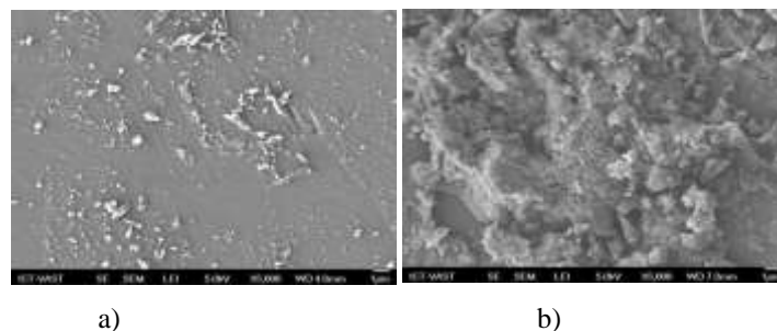
Figure 4. SEM images of (a) bare glass beads (GBs), (b) glass beads coated Ag-TiO 2 -SiO 2
