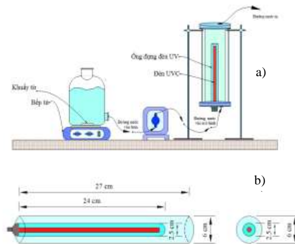
Figure 1: (a) Continuous-flow disinfection reactor used under UVC lamp and (b) UVC reactor parameters
