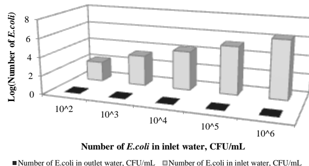
Figure 6: Effects of initial bacterial population on the photocatalytic inactivation of E.coli at 25 mL/min and pH = 6.
