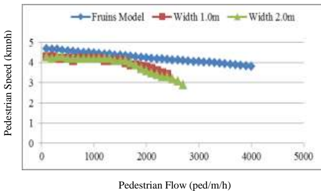
Figure 4. Pedestrian speed-flow relationship with the results of calibrated PARAMICS model plotted against Fruins models
