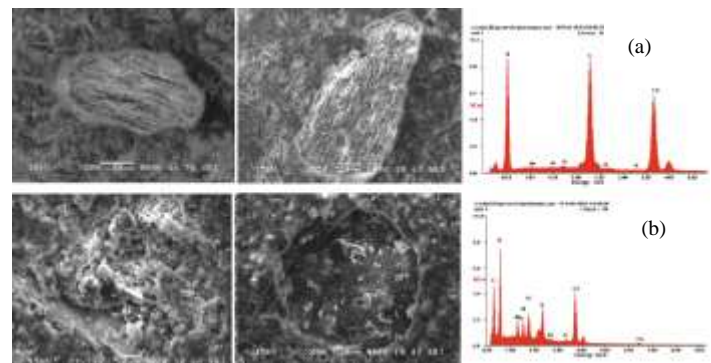
Fig. 5. SEM photograph of ettringite and thaumasite formation on the concrete communal library structure; (a) abundance presence of gypsum ; (b) the EDS spectrum shows that the height peaks for Si, S, Ca and Al, typical for thaumasite presence
