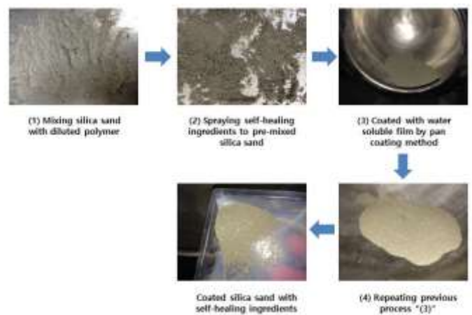
Fig.2. The method of coating and using materials.
