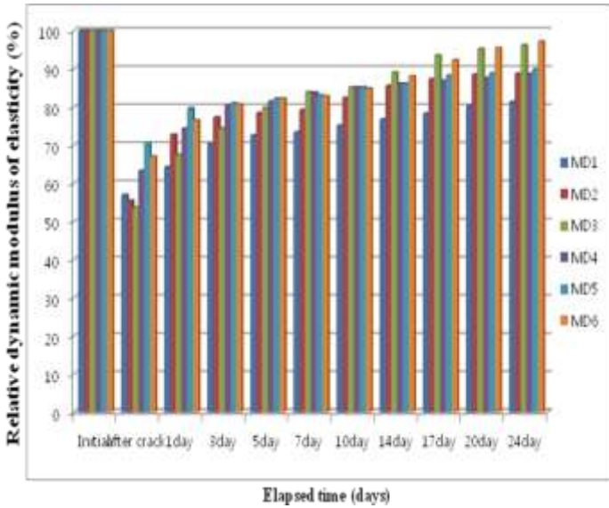
Fig. 4. Relative dynamic modulus of elasticity according to different portion of healing agent.
