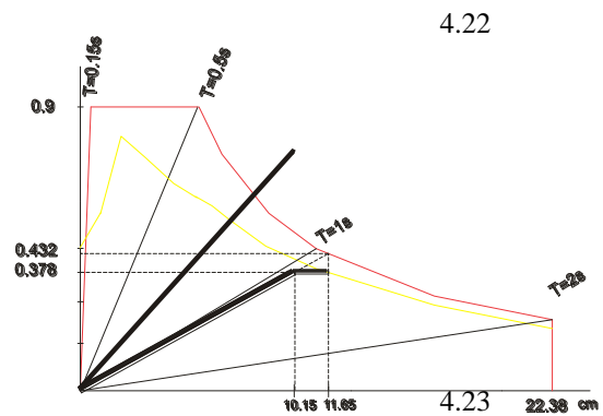
Fig.1. Displacement demand for ag=0.6g, B, EC8, v.2002
