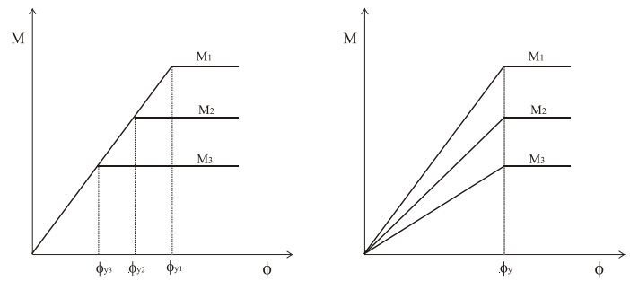
a) Constant stiffness b) constant yield curvature
