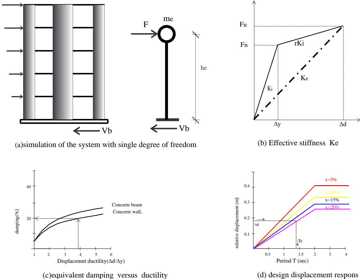
Fig. 2, Fundamentals of direct displacement based design
