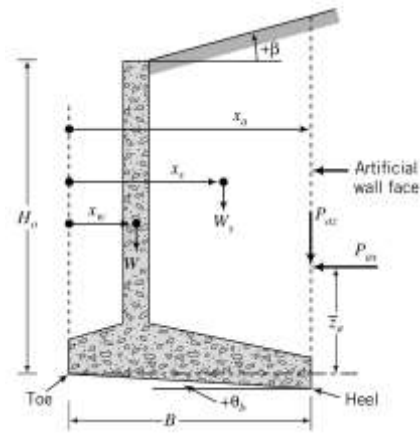
Figure 1. a typical rigid cantilever retaining wall [7]
