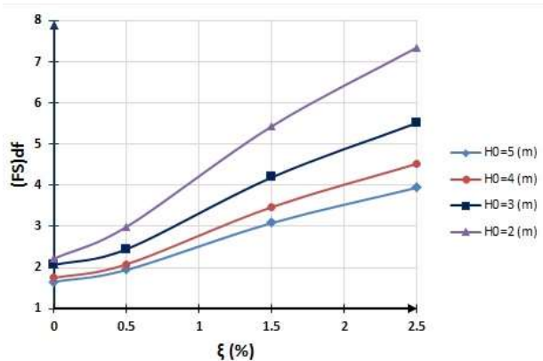
Figure 5. Factor of safety against deep-seated failure by Janbu method
