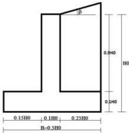
Figure 2. Geometrical properties of the rigid cantilever retaining wall Considered in the present study
