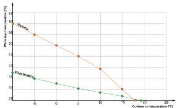
Fig.7 Floor heating temperature versus radiator heating temperature (source: drawn picture)
