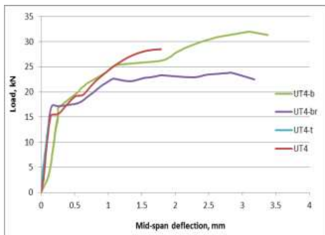
Figure 4. Load-deflection curves for different roving geometry at the same volume fraction
