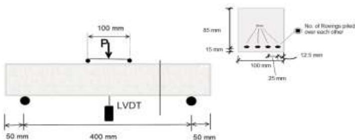
Figure 3. Four bending points test set-up, all dimensions in mm.
