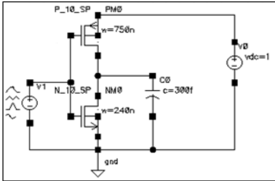
Figure 4. Inverter whose width are twice as that of reference inverter.
