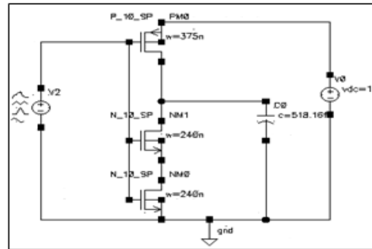
Figure 2. Inverter with series NMOS configuration.
