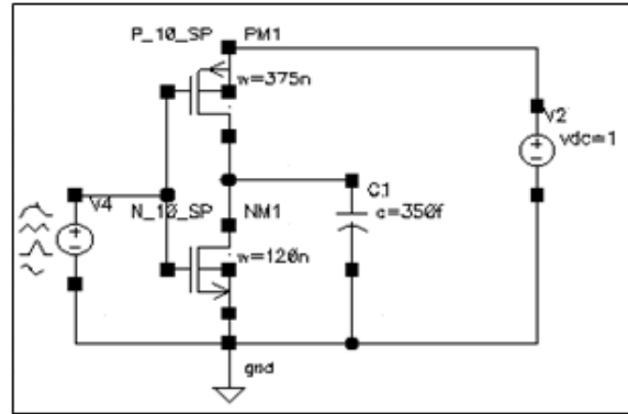
Figure 3. Circuit with h_2=1.167 \cdot h_1 of standard inverter
