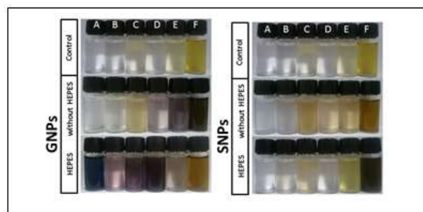
Figure 2. Snapshot of GNPs and SNPs after 1 h incubation HAuCl 4 and AgNO 3 with the following fruit extracts: A- control of 30 mM phosphate in the absence and presence of 30 mM HEPES, B- melon, C- banana, D- lemon, E- orange, F- green tea. The upper row of tubes corresponds to the synthesis in the absence of HEPES and the lower row to the synthesis in the presence of HEPES.
