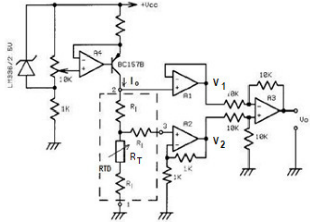
Fig. 2: Data converter unit with RTD
