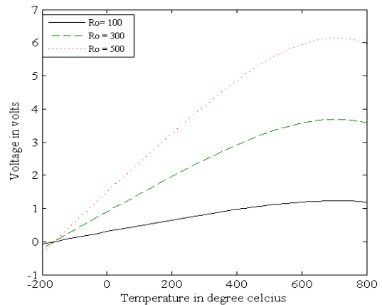
Fig.3. Output voltage for variation of temperature and R_0 , for a = 2 \times 10^{-3}, b = -5 \times 10^{-7} and c = -2 \times 10^{-12}
