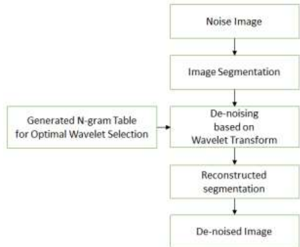
Figure 2. The de-noising procedure with n-gram table.
