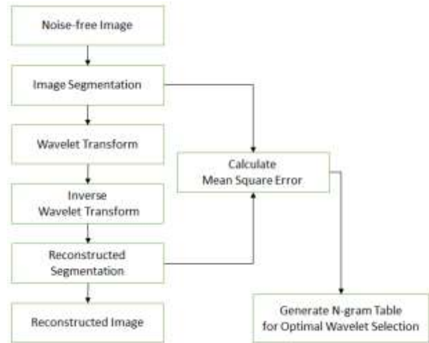
Figure 1. The wavelet function learning procedure.
