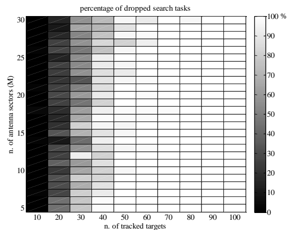
Figure 5. Percentage of dropped search tasks versus the number of tracked targets and the number of antenna sector ( M )
