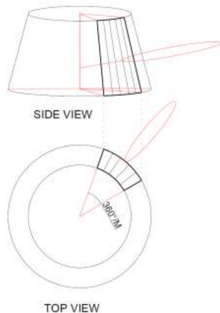
Figure 1. Conformal array (frustum of cone)
