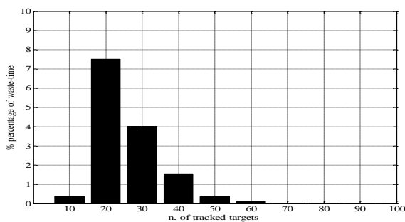
Figure 8. Percentage of waste time versus n. of tracked targets
