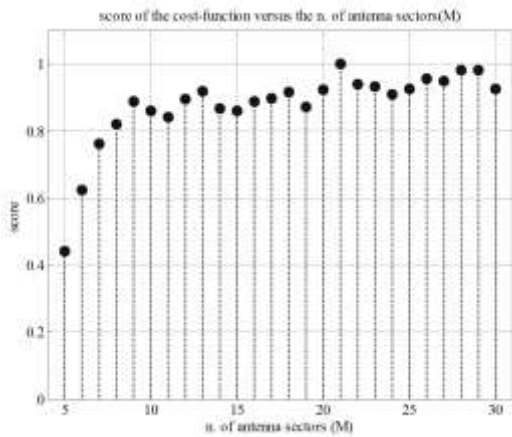
Figure 7. Score of the results cost-function versus the number of antenna sector ( M )
