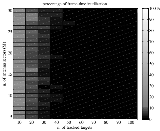
Figure 6. Percentage of not-used time-frame versus the number of tracked targets and the number of antenna sector ( M )
