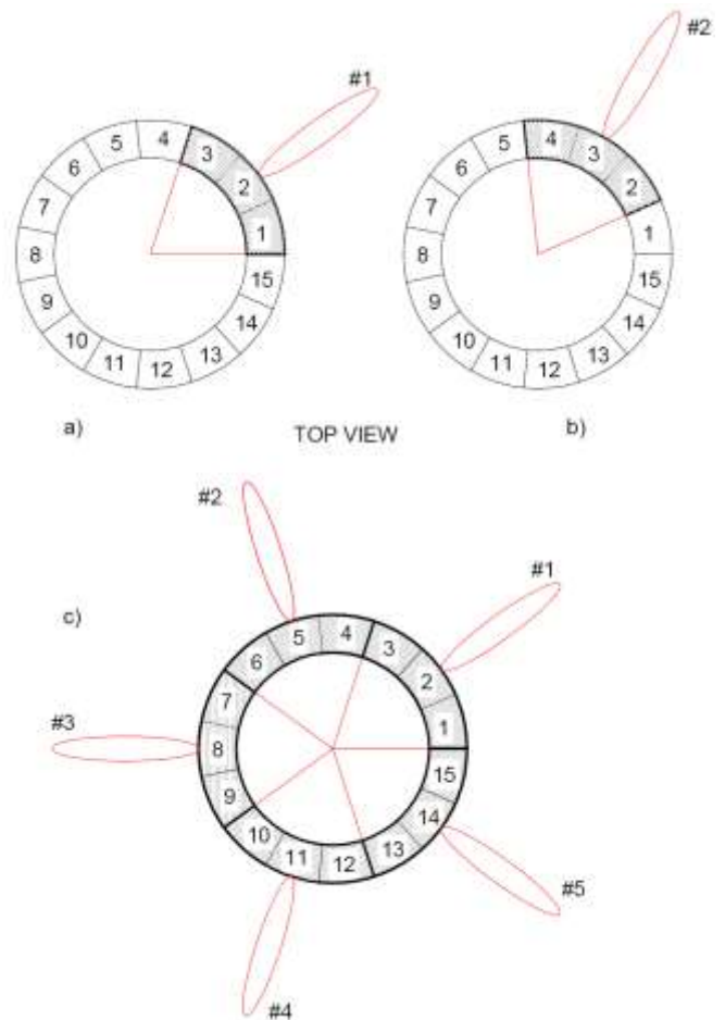
Figure 2. Antenna sectors division: a) beam of the sub-array #1, columns: [1-2-3], b) beam of the sub-array #2, columns: [2-3-4], sub-array #1 and #2 are overlapped and they can not transmit simultaneously (they have common columns: [2, 3]); c) antenna sectors division for search function, sub-arrays #1, #2, #3 #4 and #5 are not-overlapping, and can transmit/receive simultaneously
