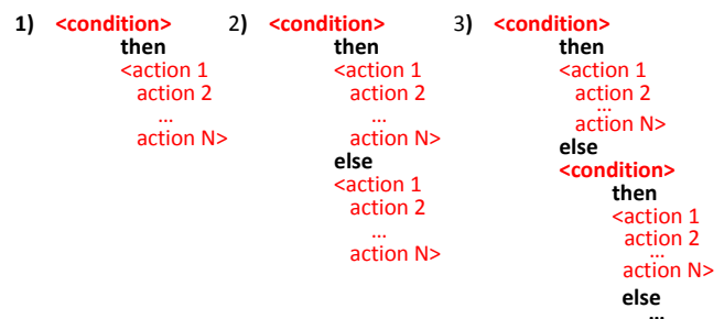
Figure 1. Basic types of Condition and Action Business rules
