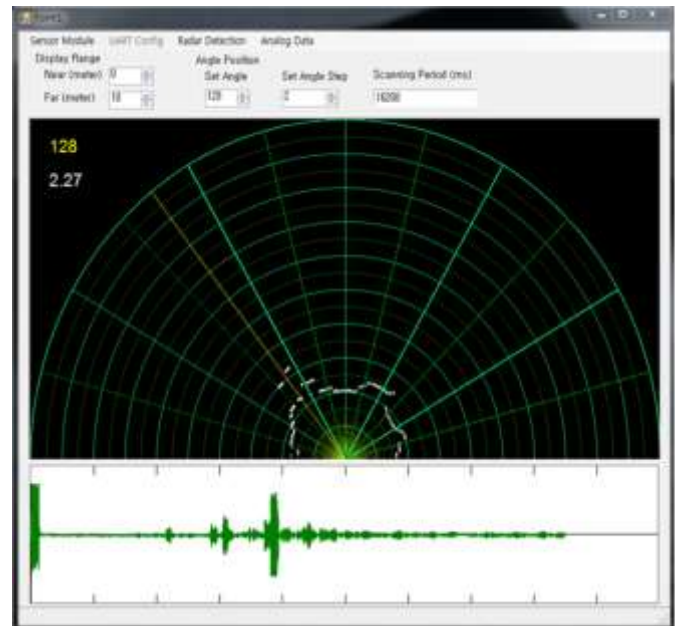
Figure 7: GUI and Display of PC based Target Area
