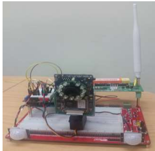
Figure 3: Motion detection and image capture system
