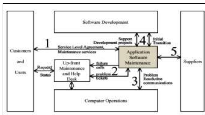
Figure 1. Software Maintenance Context Diagram
