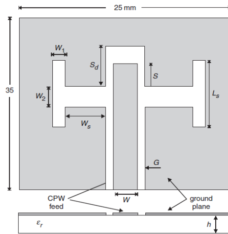
Figure4.Geometry of CPW-fed capacitive H-shaped slot antenna
