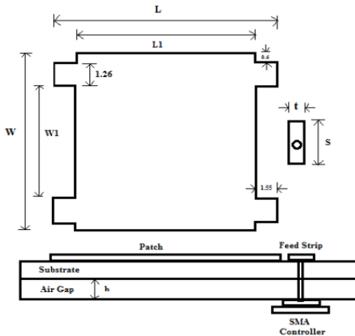
Figure 3 Capacitive feed H Patch antenna
