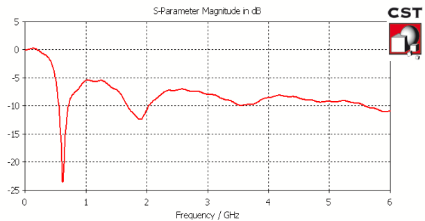
Fig. 2 Return loss for b = 85 mm
