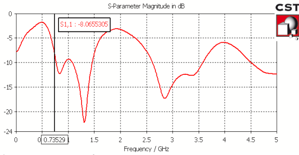
Fig. 3 Return Loss for r = 0\text{mm}
