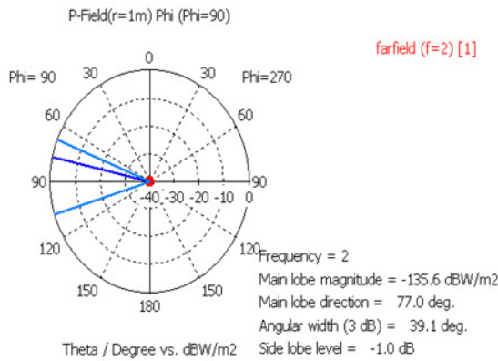
Fig. 15 Cross polarization pattern in E-Plane at f = 2 GHz
