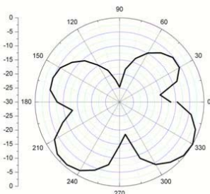
Fig.11 Measured Radiation Pattern in E-Plane at f=2 GHz
