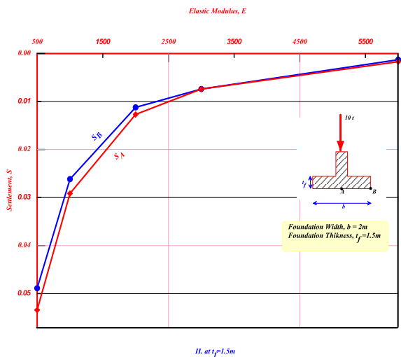
Figure4: Relationship between settlement and elastic modulus in clay only
