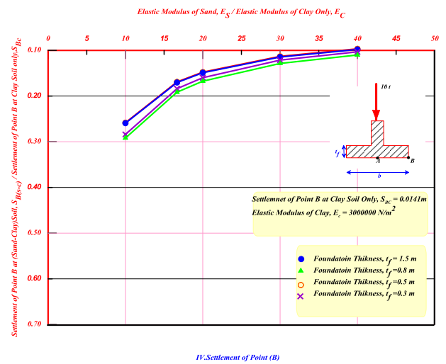
Figure 5: Relationship Between Point (A) and (B) Settlement and E_{sand}/E_{clay} at E_c = 2 , and 3 (MN/m 2 ).
