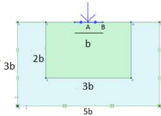
Figure 2: Case of clay with geocell sand without geogrid
