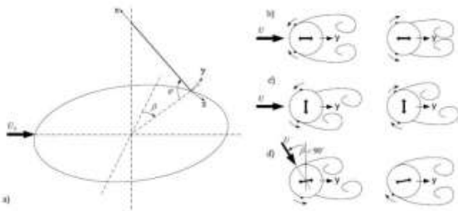
Figure 2. Effect of the yaw angle \beta (Jensen & Gadegaard, 2009).
