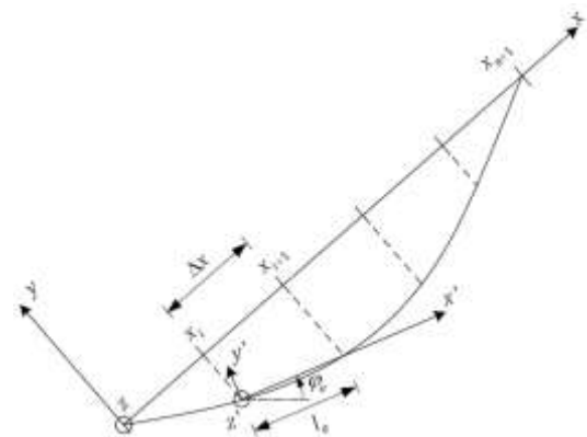
Figure 4. Stay cable model.
