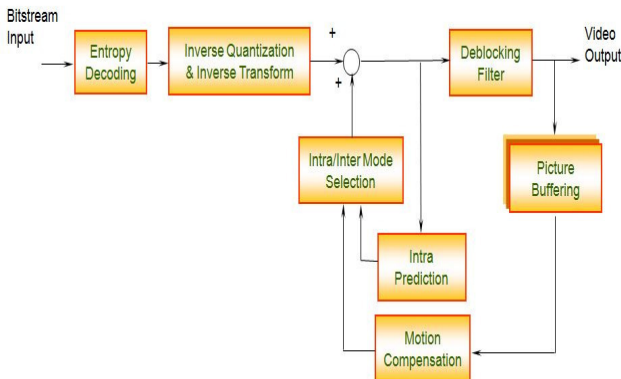
Fig. 2: H.264 decoder block diagram.
