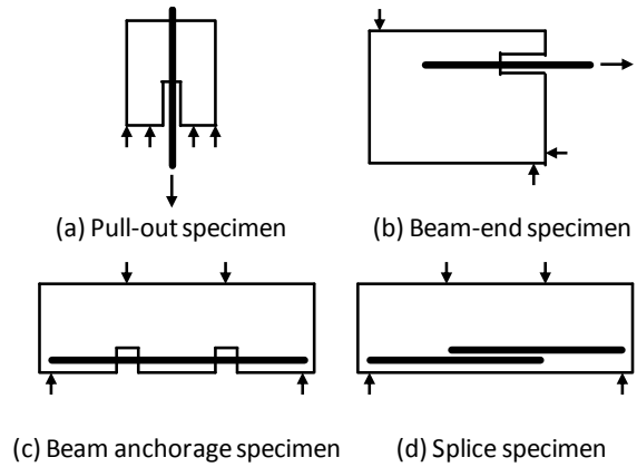
Figure 1. Bond strength test specimens
