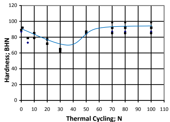
Figure 4. Effect of thermal fatigue on hardness at temperature; T_h = 100 °C.
