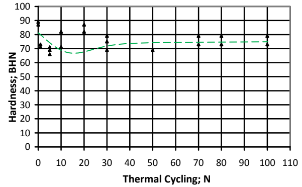
Figure 6. Effect of thermal fatigue on hardness at temperature; T_h = 500^\circ\text{C}
