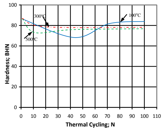
Figure 7. Comparison of thermal fatigue on hardness at different values of heating temperature; T_h = 100, 300 and 500 °C
