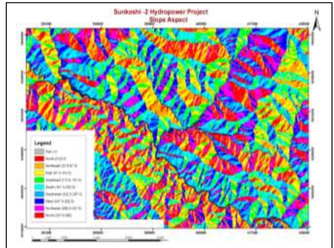
Figure 5: Slope Aspect Map of the project area
