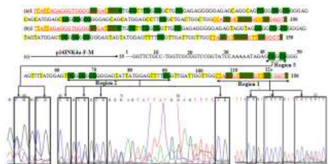
Figure 2. Sequencing profile of methylated of p16^{INK4a} . (CG sites were in the green highlight; Cytosine did not depend on the CpG site were in yellow. (a) DNA sequence was without bisulfite modified; (b) DNA
