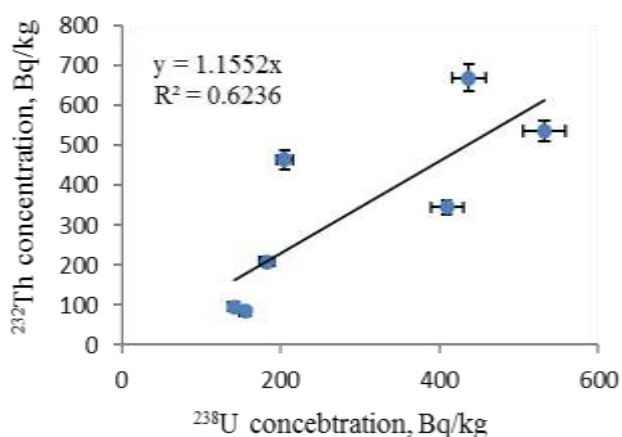
Fig. 3. Correlation between 238 U and 232 Th in the analyzed rock samples.
