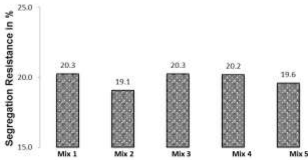
Figure 6. Sieve Segregation Resistance Test
