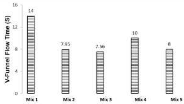
Figure 4: V-Funnel Flow Time Test results
