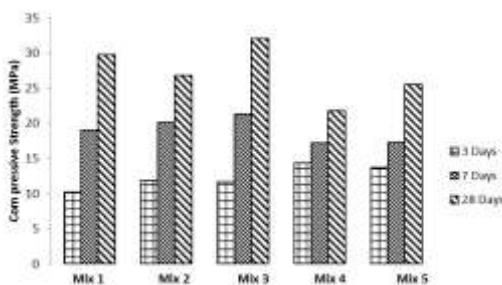
Figure 7. Compressive Strength of Mixes
