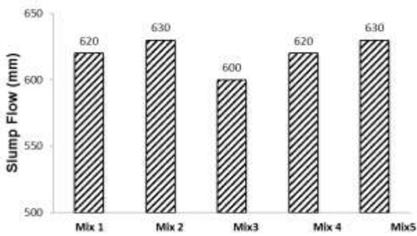
Figure 2: Slump Test results
