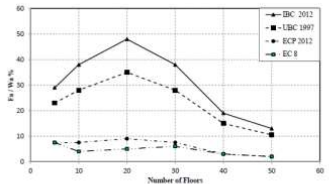
Figure 6. Percentage of nonstructural seismic force to weight ratio using (nonstructural element at 5 th floor and T_a=0.07 sec).
