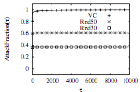
(b) AttackFraction(\tau)
