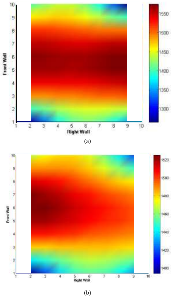
Figure 6. Temperature profiles taken at 33 m for coal B (a) before and (b) after coal mills were switched.
