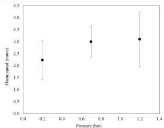
Figure 7. Approximate flame speeds vs variation in furnace pressure
