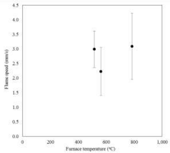
Figure 5. Approximate flame speeds vs furnace temperature
