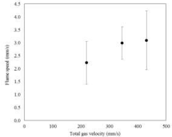
Figure 6. Approximate flame speeds vs total gas velocity
