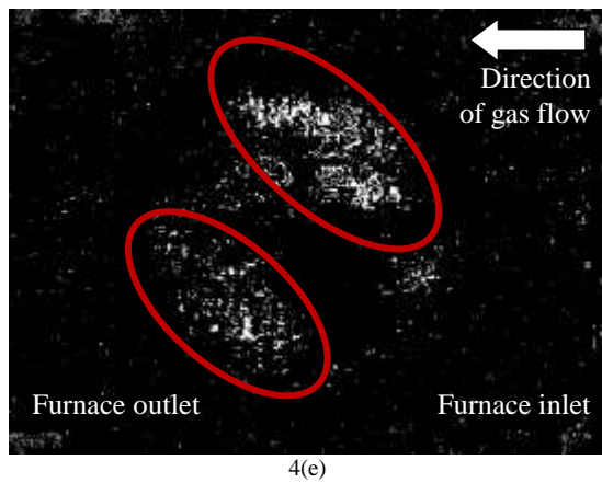
Figure 4. (a) and (b) two subsequent infrared images (c) and (d) images in 32-bit format (e) subtracted and threshold adjusted image. Circled areas indicate pixels with the largest difference in brightness.
