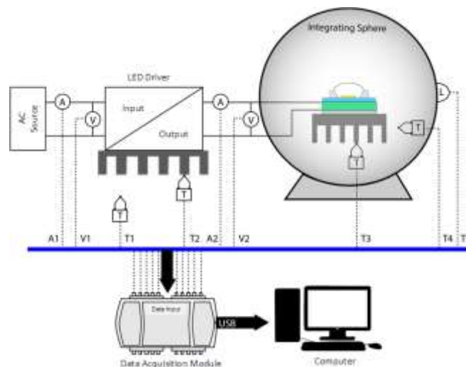
Figure 4. Experimental setup of LED luminaire test system.
