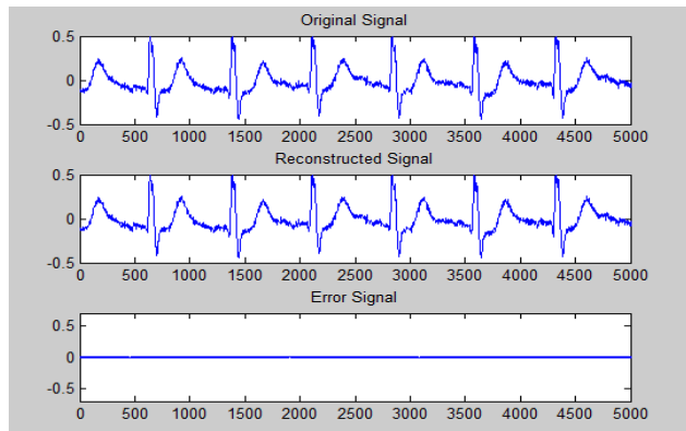
Fig. 7 Wavelet Transform
