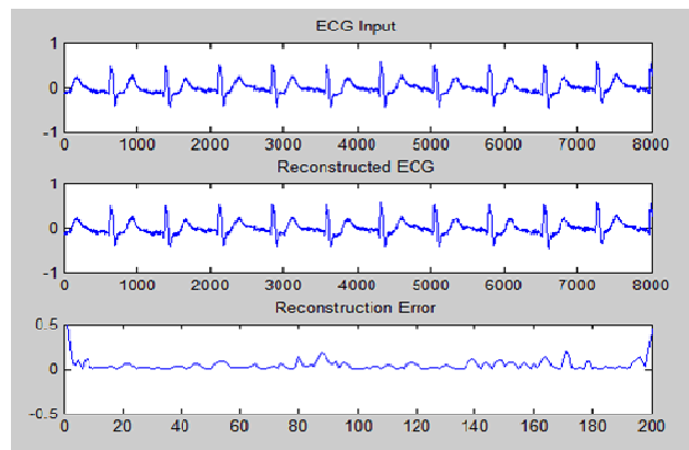
Fig. 6 Walsh Transform
