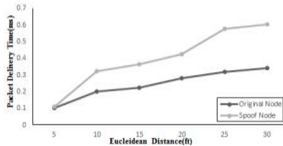
Figure 7. Packet delivery time vs Euclidean distance
