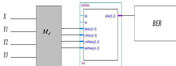
Figure 7. FPGA Architecture of 3dimensional Turbo Decoder
