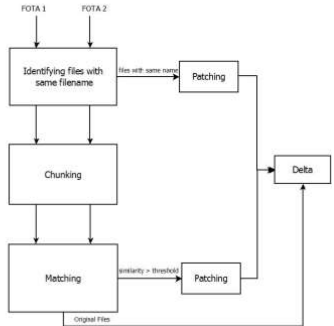
Figure 1: Overall algorithm pipeline
