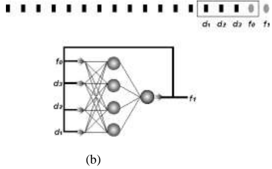
Figure 4 Iteratively forecasting (a) the first forecast and (b) the second forecast. This figure corresponds to Fig.3 (a).
