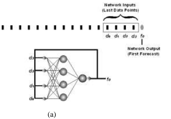
Figure 3 Creating examples with a moving window for a network with four inputs and one output. In (a), the step-ahead size is 1; in (b), the step-ahead size is 4.
