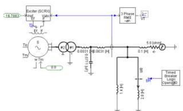
Figure.6. System Under Study(after compensation)
