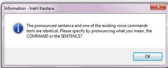
Figure 4. Information messagebox.
