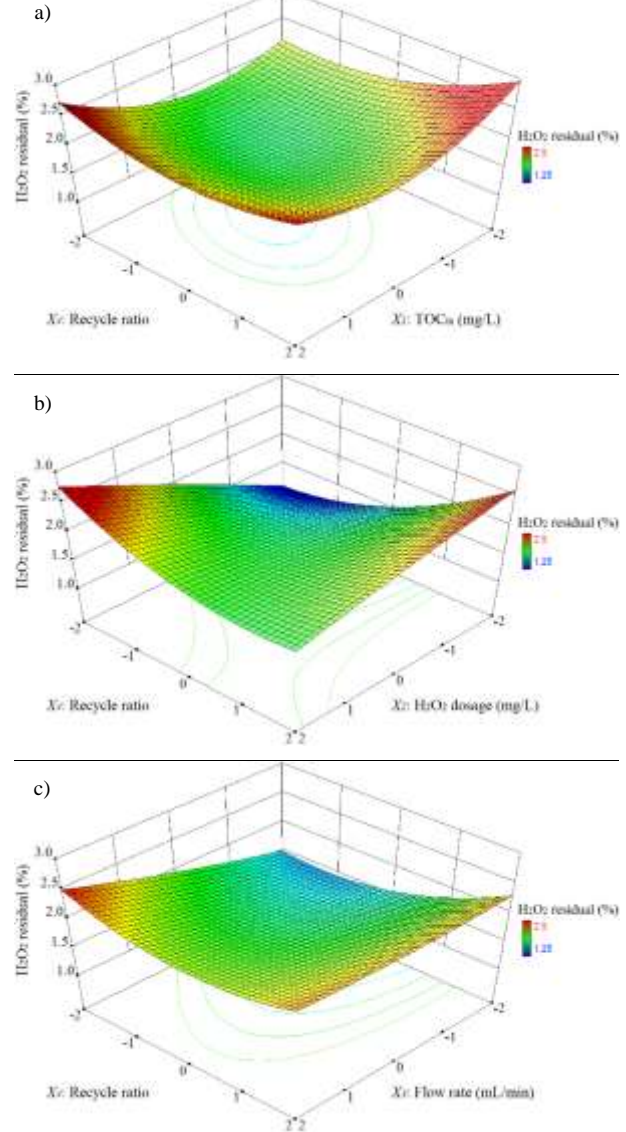
Figure 4. Interaction effects of different parameters on the H_2O_2 residual using 3D response surface and 2D contours: (a) influent concentration of TOC and recycle ratio ( X_1X_4 ), (b) H_2O_2 dosage and recycle ratio ( X_2X_4 ), and (c) flow rate and recycle ratio ( X_3X_4 ).
