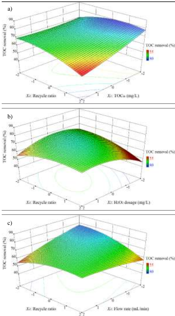
Figure 3. Interaction effects of different parameters on the percent TOC removal using 3D response surface and 2D contours: (a) influent concentration of TOC and recycle ratio ( X_1X_4 ), (b) H_2O_2 dosage and recycle ratio ( X_2X_4 ), and (c) flow rate and recycle ratio ( X_3X_4 ).
