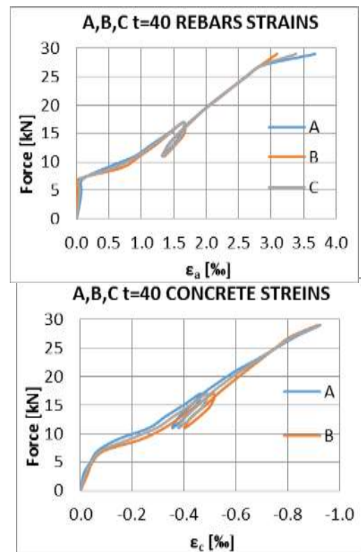
Fig. 4. Comparing the diagrams of strains in concrete and reinforcement – Series: A, B, C, t=40 days
