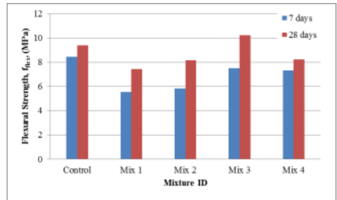
Figure 4. The effect of plastic particles on the flexural strength of SCC mixtures
