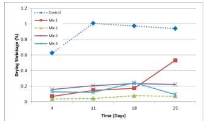
Figure 2. The effect of plastic particles on drying shrinkage
