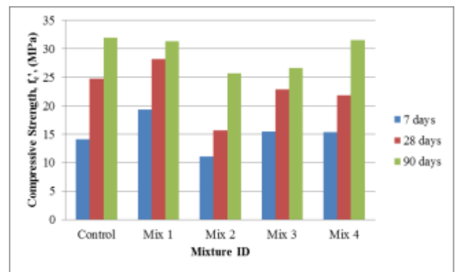
Figure 3. The effect of plastic particles on the compressive strength of SCC mixtures
