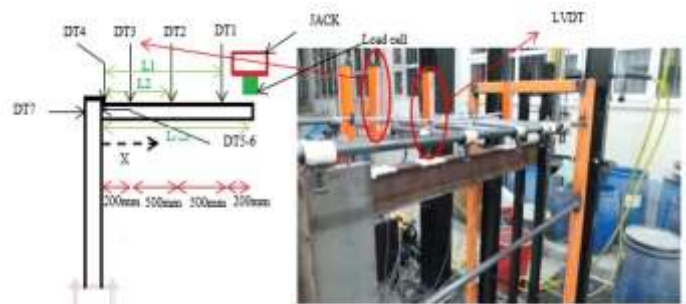
Fig. 2. Location of the displacement transducers (DT=LVDTs)
