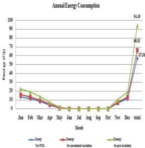
Fig.4. Annual energy consumption in each condition.
