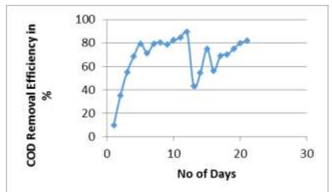
Fig.6. COD removal efficiency vs no of days .
