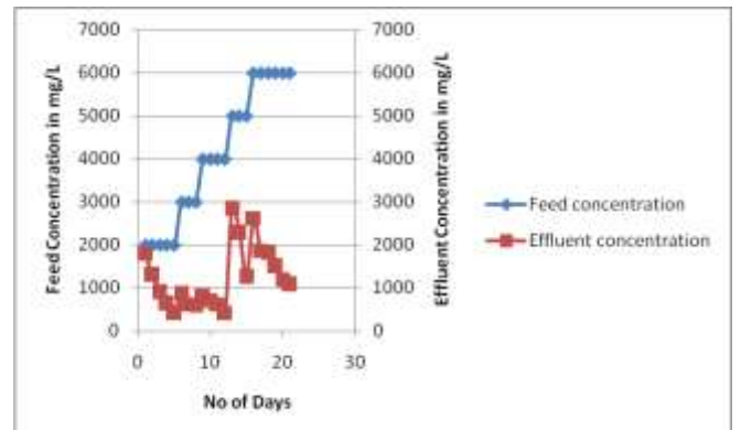
Fig. 4. Correlation between Feed Concentration and Effluent Concentration.
