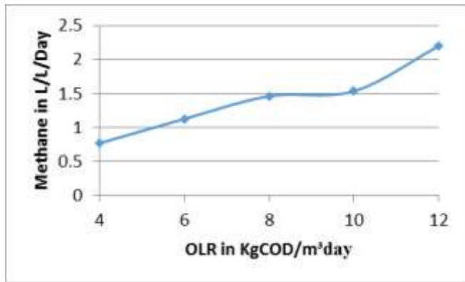
Fig.7. Methane production. vs OLR .
