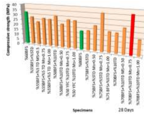
Figure5. A graph of the compressive strength of the tile dust content specimens at 28 days
