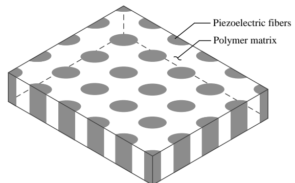
Figure 1. Schematic of a 1-3 piezocomposite
