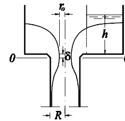
Figure 1: Configuration of the Drioli vortex-flow inlet.
