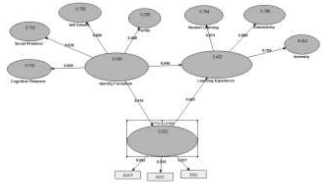
Fig. 3: Measurement Model
